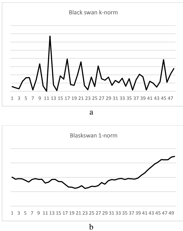
Fig. 2 Ky Fan norm fluctuations for k-norm (a) and 1-norm (b)
