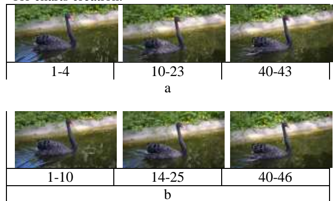
Fig. 1. Key frames detected manually (a) and by the developed system (b)
